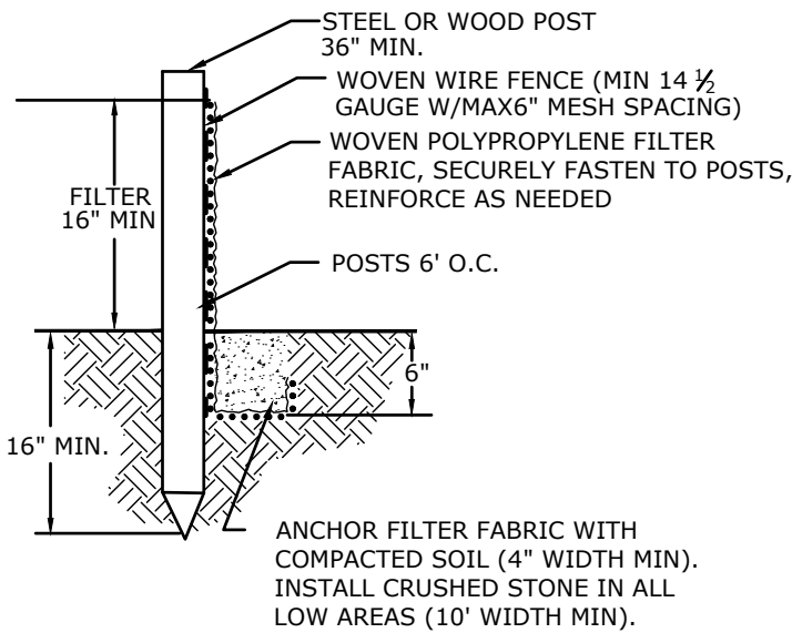
TRENCHED INSTALLATION
